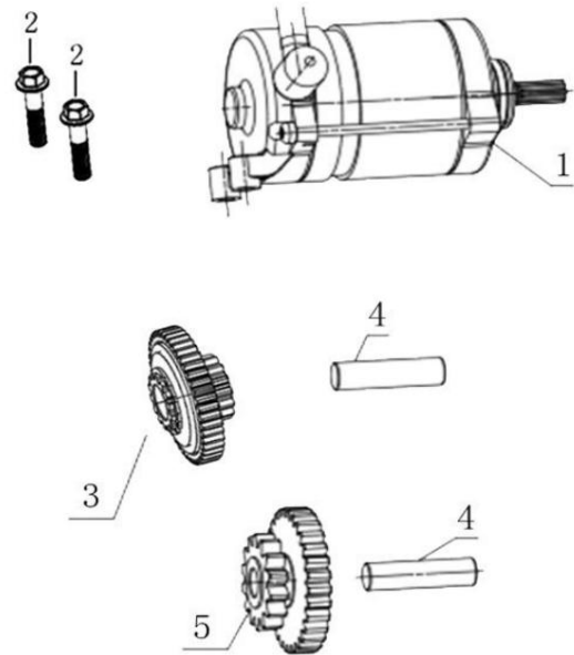
电启动机构 ELECTRIC STARTING MECHANI
