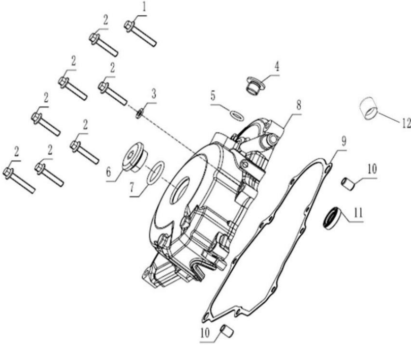
左曲轴箱盖 LEFT CRANKCASE COVER
