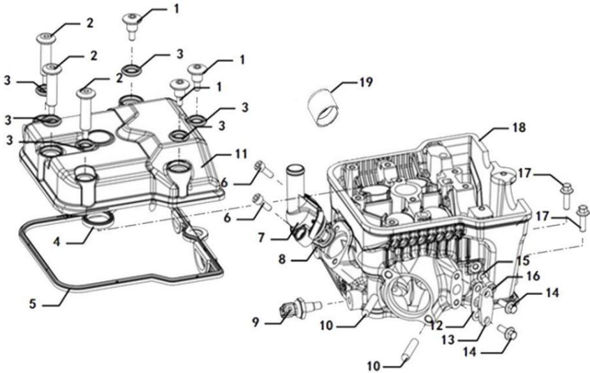
气缸头部件 CYLINDER HEAD ASSY
