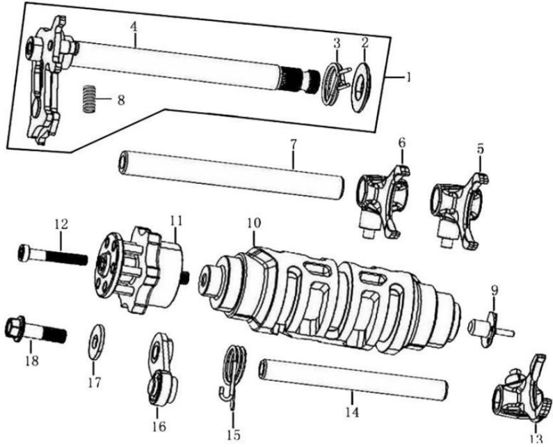
变速机构 GEARSHIFT MECHANISM
